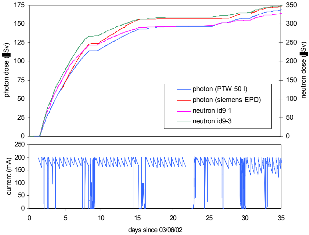
Figure 8: Neutron and photon dose outside the ID9 optics hutch during 5 weeks of operation.
